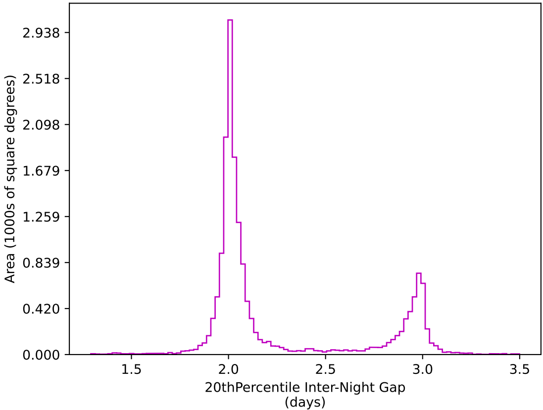
ddf_acor_sf10_lsf15_lsr10_v3.4_10yrs WFD z band: 20thPercentile Inter-Night Gap
