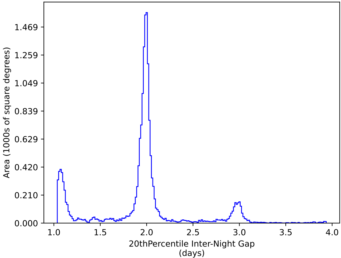
ddf_acor_sf10_lsf15_lsr10_v3.4_10yrs WFD y band: 20thPercentile Inter-Night Gap
