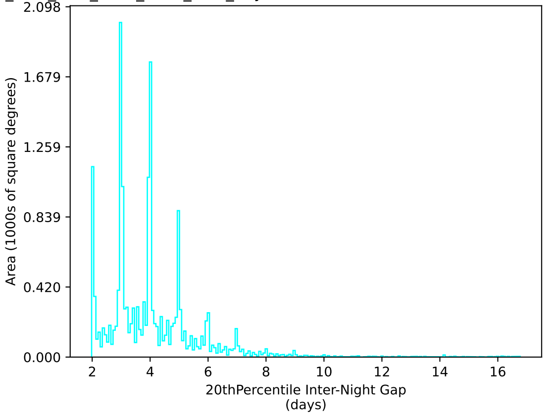
ddf_acor_sf10_ls15_lsr10_v3.4_10yrs WFD u band: 20thPercentile Inter-Night Gap
