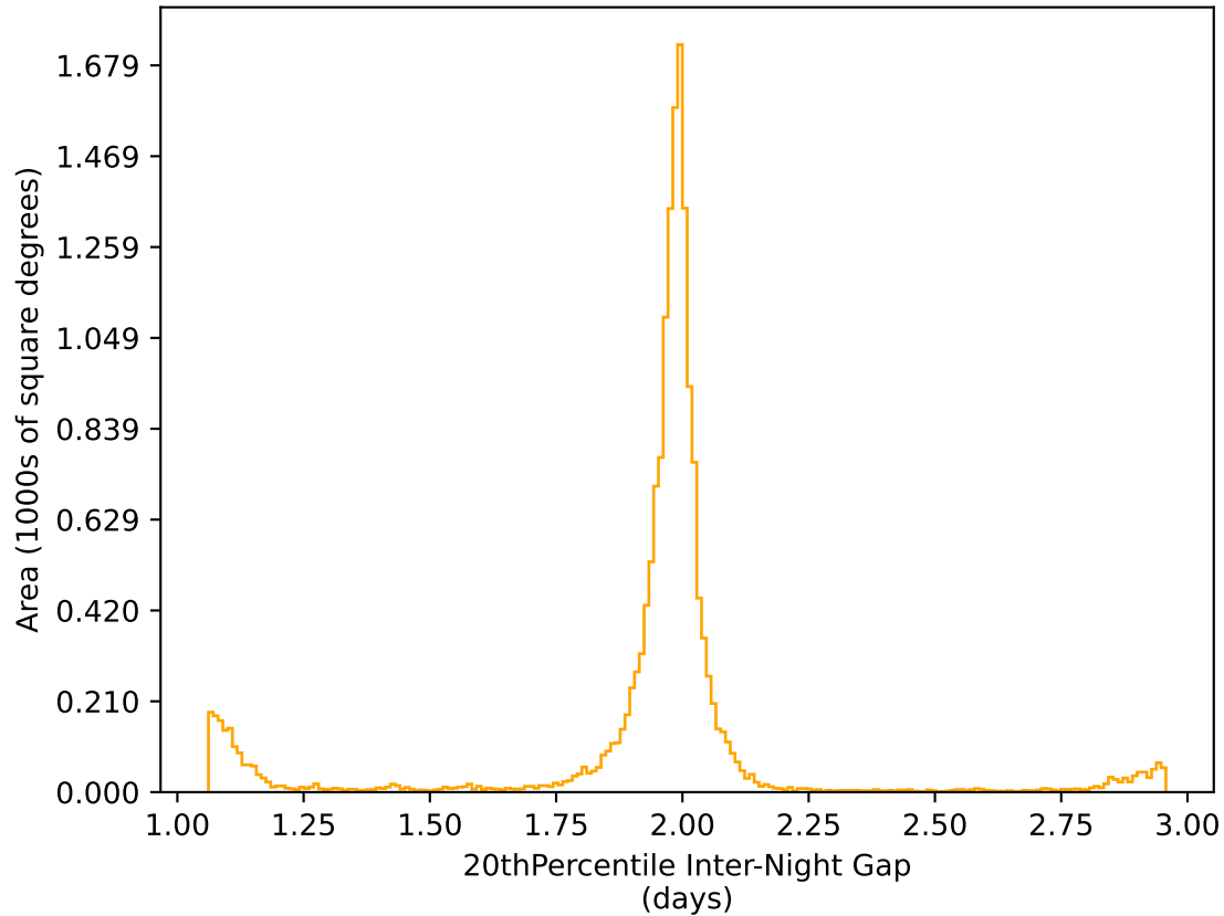
ddf_acor_sf10_lsf15_lsr10_v3.4_10yrs WFD r band: 20thPercentile Inter-Night Gap
