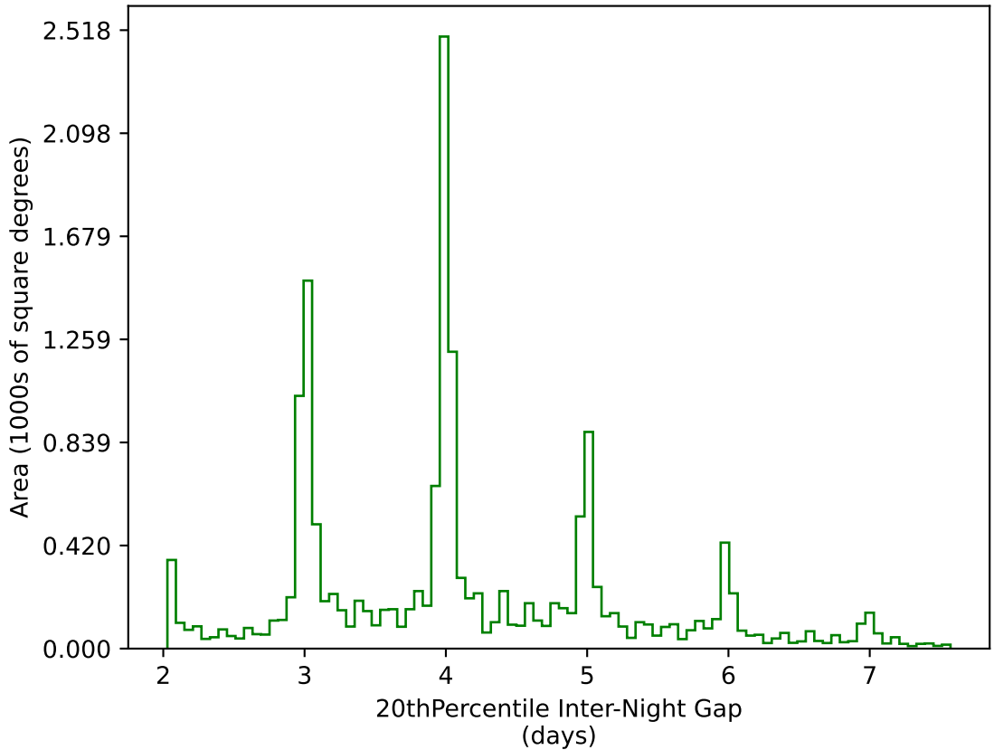
ddf_acor_sf10_lsf15_lsr10_v3.4_10yrs WFD g band: 20thPercentile Inter-Night Gap
