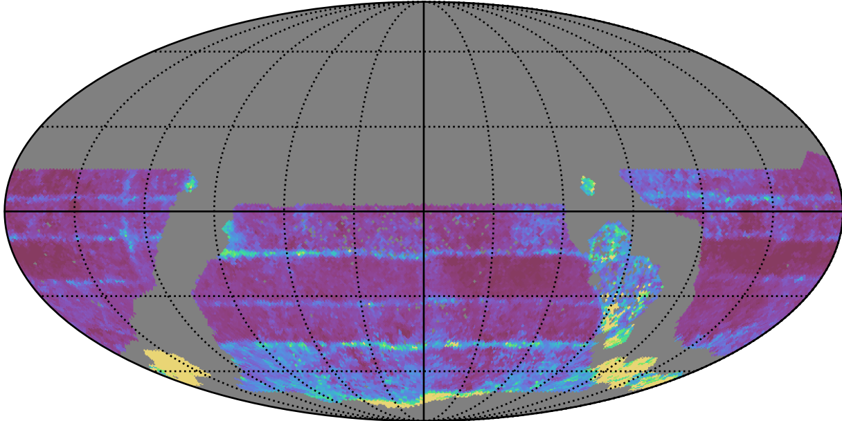
ddf_acor_sf10_lsf15_lsr10_v3.4_10yrs WFD all bands: 20thPercentile Inter-Night Gap
