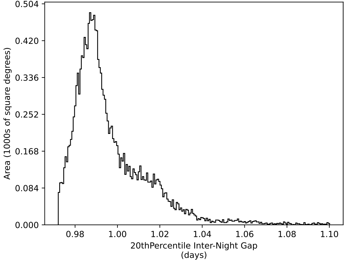
ddf_acor_sf10_ls15_lsr10_v3.4_10yrs WFD all bands: 20thPercentile Inter-Night Gap
