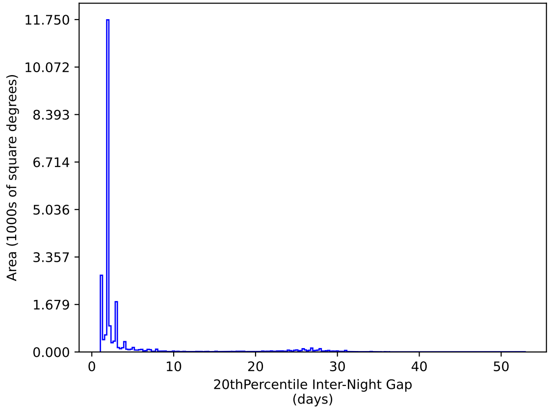
ddf_acor_sf10_ls15_lsr10_v3.4_10yrs All sky y band: 20thPercentile Inter-Night Gap
