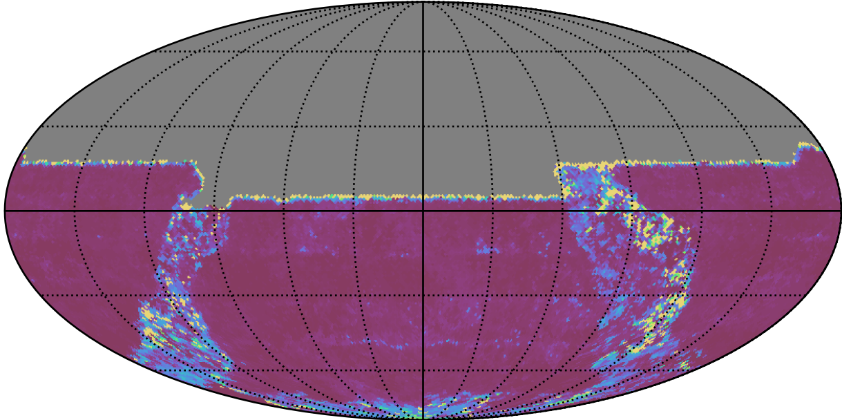
ddf_acor_sf10_lsf15_lsr10_v3.4_10yrs All sky u band: 20thPercentile Inter-Night Gap
