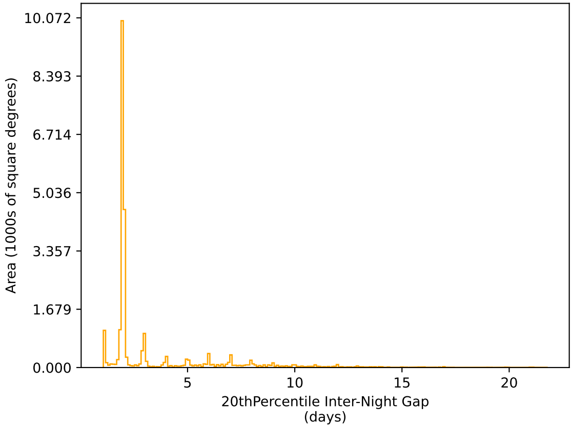
ddf_acor_sf10_ls15_lsr10_v3.4_10yrs All sky r band: 20thPercentile Inter-Night Gap
