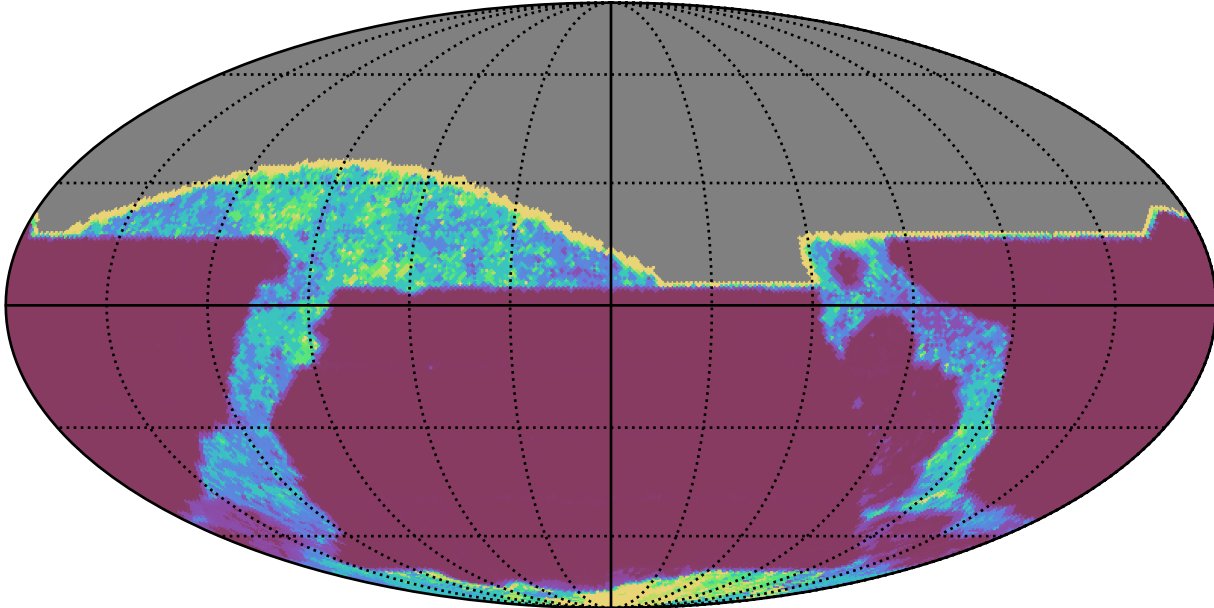
ddf_acor_sf10_lsf15_lsr10_v3.4_10yrs All sky all bands: 20thPercentile Inter-Night Gap
