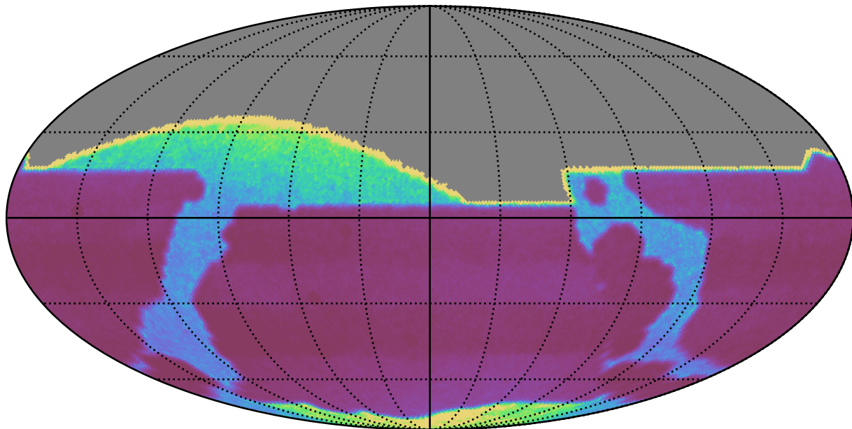
ddf_acor_sf10_lsf15_lsr10_v3.4_10yrs : properMotion
