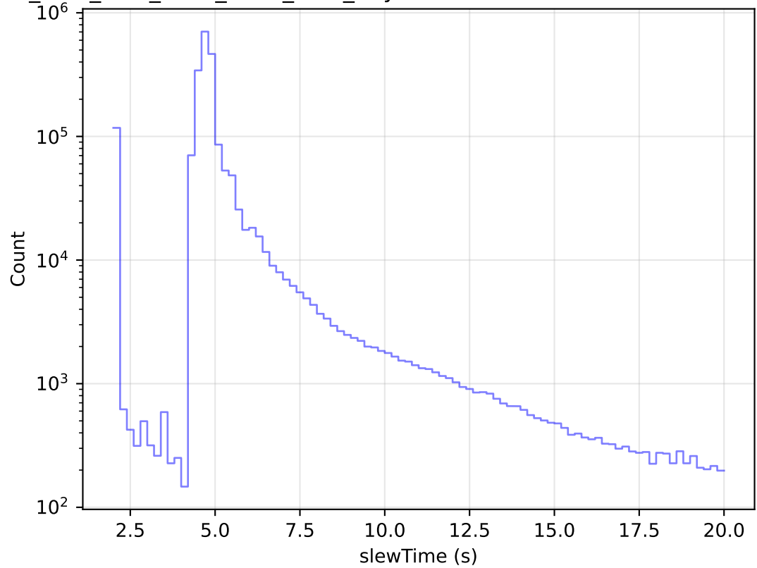
ddf_acor_sf10_Isf15_Isr10_v3.4_10yrs All visits: Zoom Slew Time Histogram
