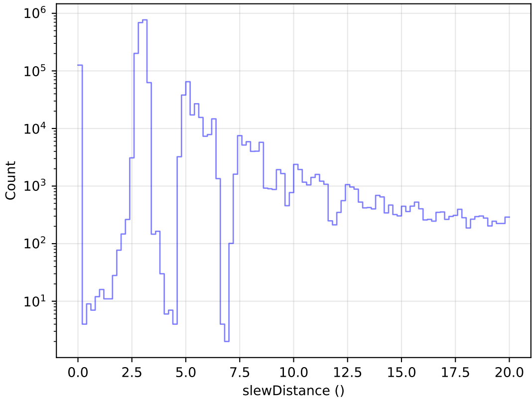
ddf_acor_sf10_lsf15_lsr10_v3.4_10yrs All visits: Zoom Slew Distance Histogram
