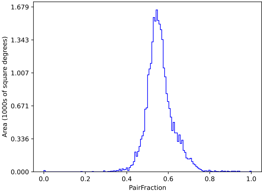
ddf_acor_sf10_lsf15_lsr10_v3.4_10yrs (g or r or i): PairFraction
