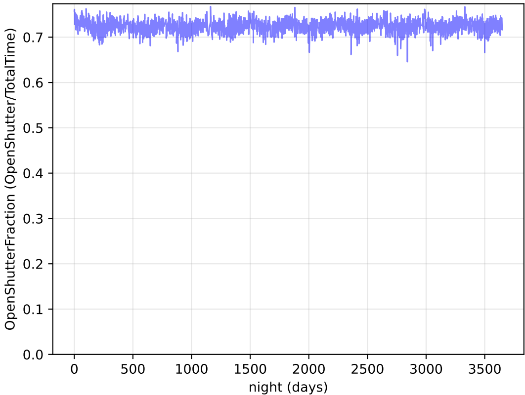
ddf_acor_sf10_lsf15_lsr10_v3.4_10yrs : OpenShutterFraction
