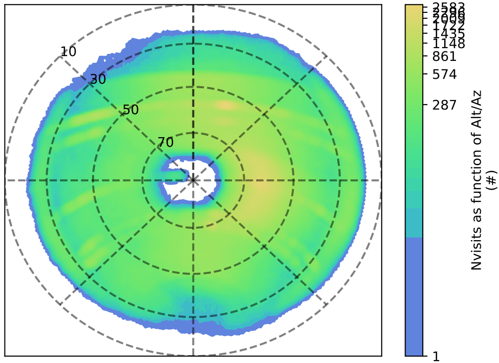
ddf_acor_sf10_lsf15_lsr10_v3.4_10yrs z: Nvisits as function of Alt/Az
