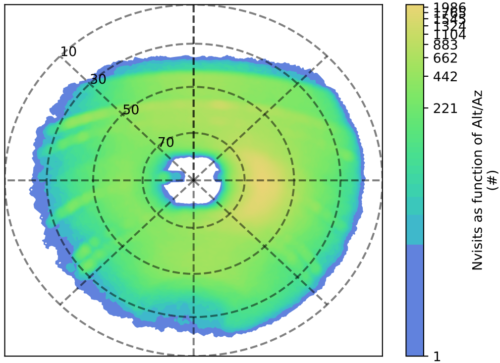
ddf_acor_sf10_ls15_lsr10_v3.4_10yrs y: Nvisits as function of Alt/Az
