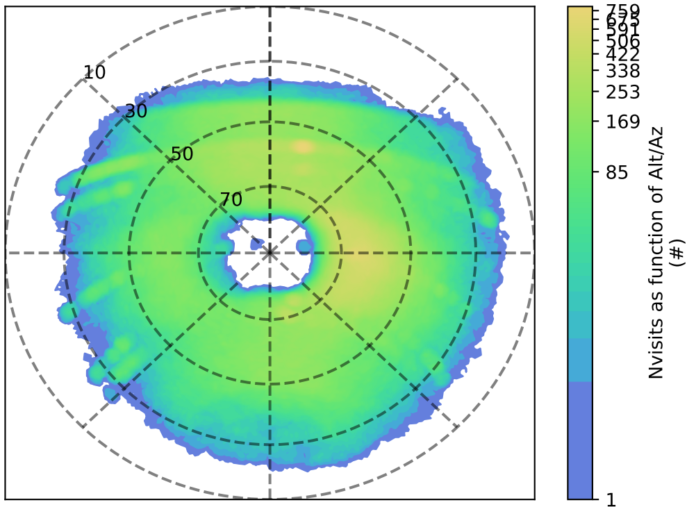
ddf_acor_sf10_ls15_lsr10_v3.4_10yrs u: Nvisits as function of Alt/Az
