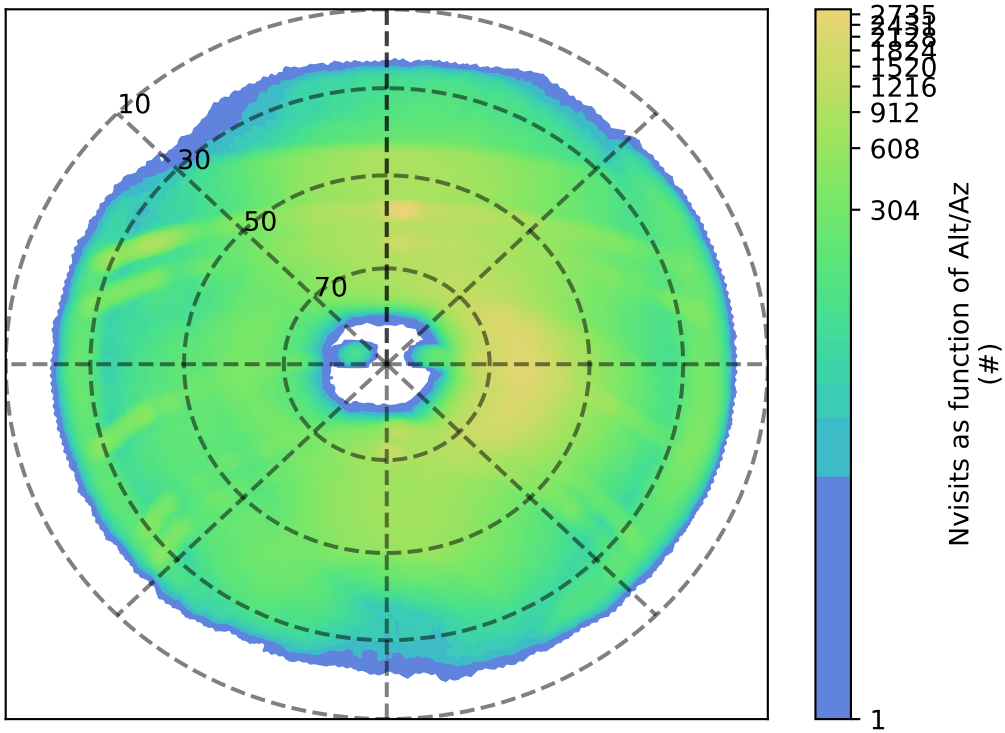
ddf_acor_sf10_ls15_lsr10_v3.4_10yrs i: Nvisits as function of Alt/Az
