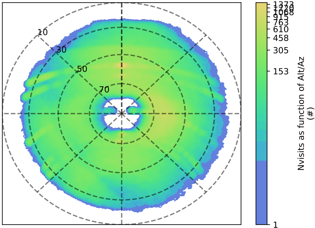
ddf_acor_sf10_lsf15_lsr10_v3.4_10yrs g: Nvisits as function of Alt/Az
