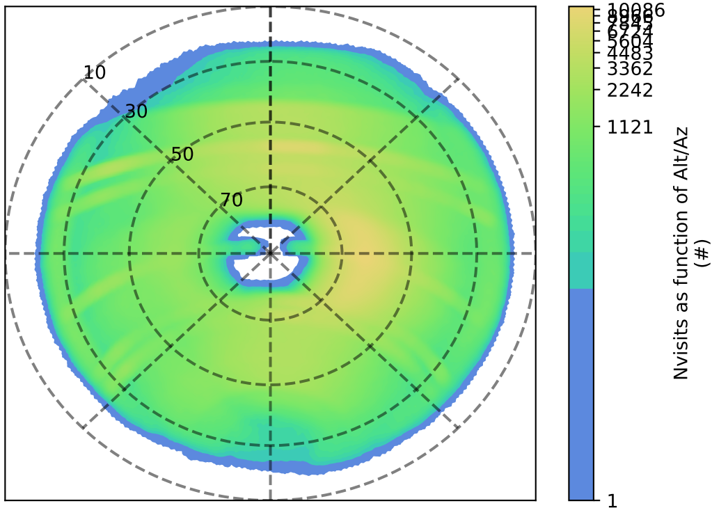
ddf_acor_sf10_lsf15_lsr10_v3.4_10yrs : Nvisits as function of Alt/Az
