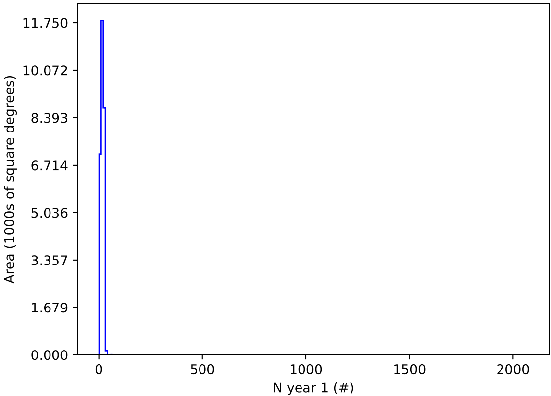
ddf_acor_sf10_lsf15_lsr10_v3.4_10yrs i and night < 365: N year 1
