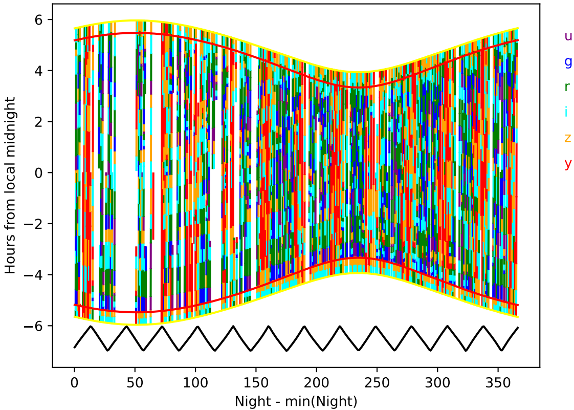
ddf_acor_sf10_lsf15_lsr10_v3.4_10yrs year 8-9: Hourglass
