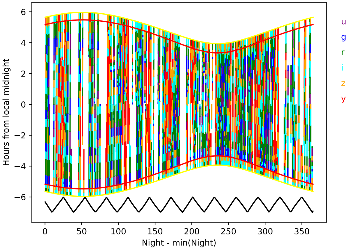
ddf_acor_sf10_lsf15_lsr10_v3.4_10yrs year 7-8: Hourglass
