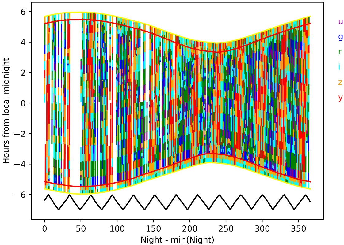
ddf_acor_sf10_lsf15_lsr10_v3.4_10yrs year 6-7: Hourglass
