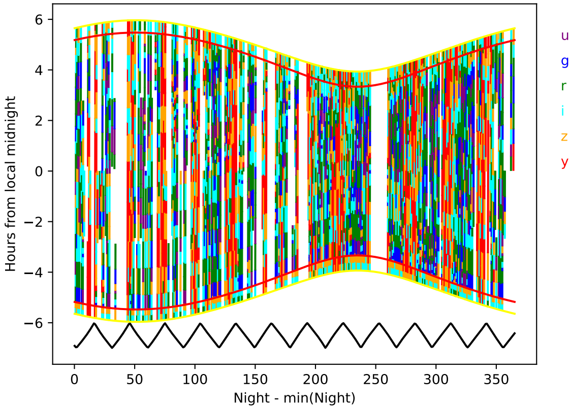
ddf_acor_sf10_lsf15_lsr10_v3.4_10yrs year 5-6: Hourglass
