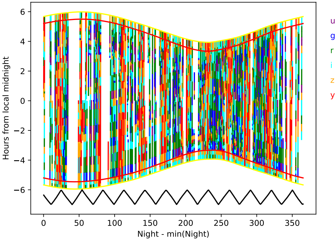
ddf_acor_sf10_lsf15_lsr10_v3.4_10yrs year 4-5: Hourglass
