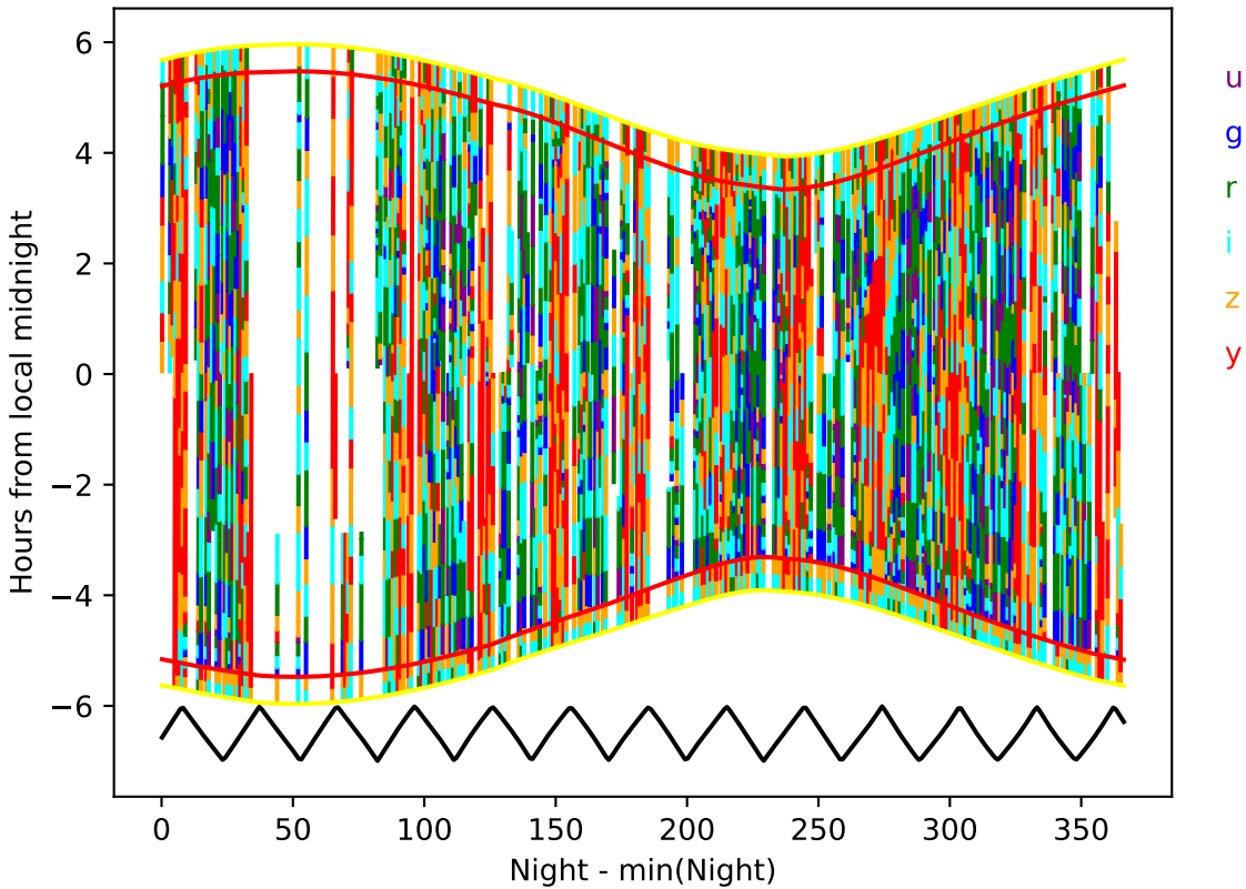
ddf_acor_sf10_lsf15_lsr10_v3.4_10yrs year 3-4: Hourglass
