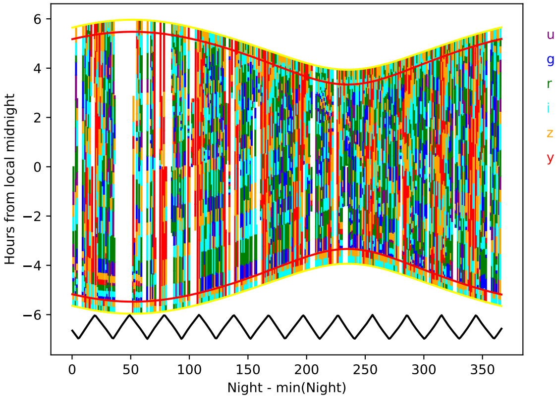
ddf_acor_sf10_ls15_lsr10_v3.4_10yrs year 2-3: Hourglass
