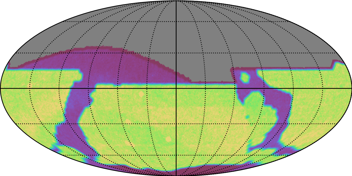
ddf_acor_sf10_lsf15_lsr10_v3.4_10yrs : Count observationStartMJD
