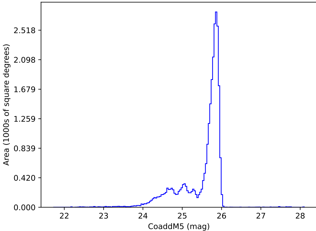
ddf_acor_sf10_ls15_lsr10_v3.4_10yrs z: CoaddM5
