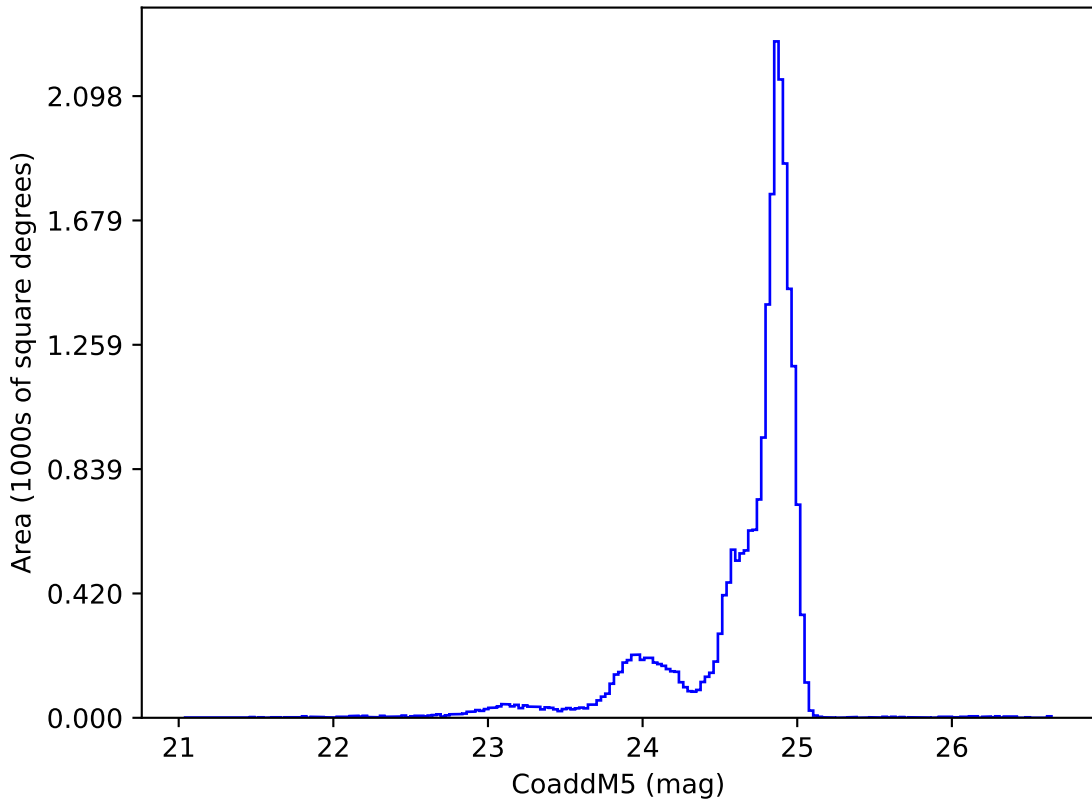
ddf_acor_sf10_lsf15_lsr10_v3.4_10yrs y: CoaddM5
