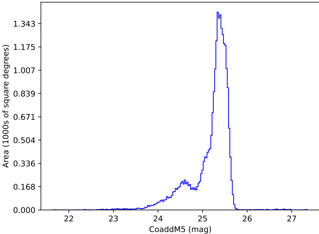
ddf_acor_sf10_lsf15_lsr10_v3.4_10yrs u: CoaddM5
