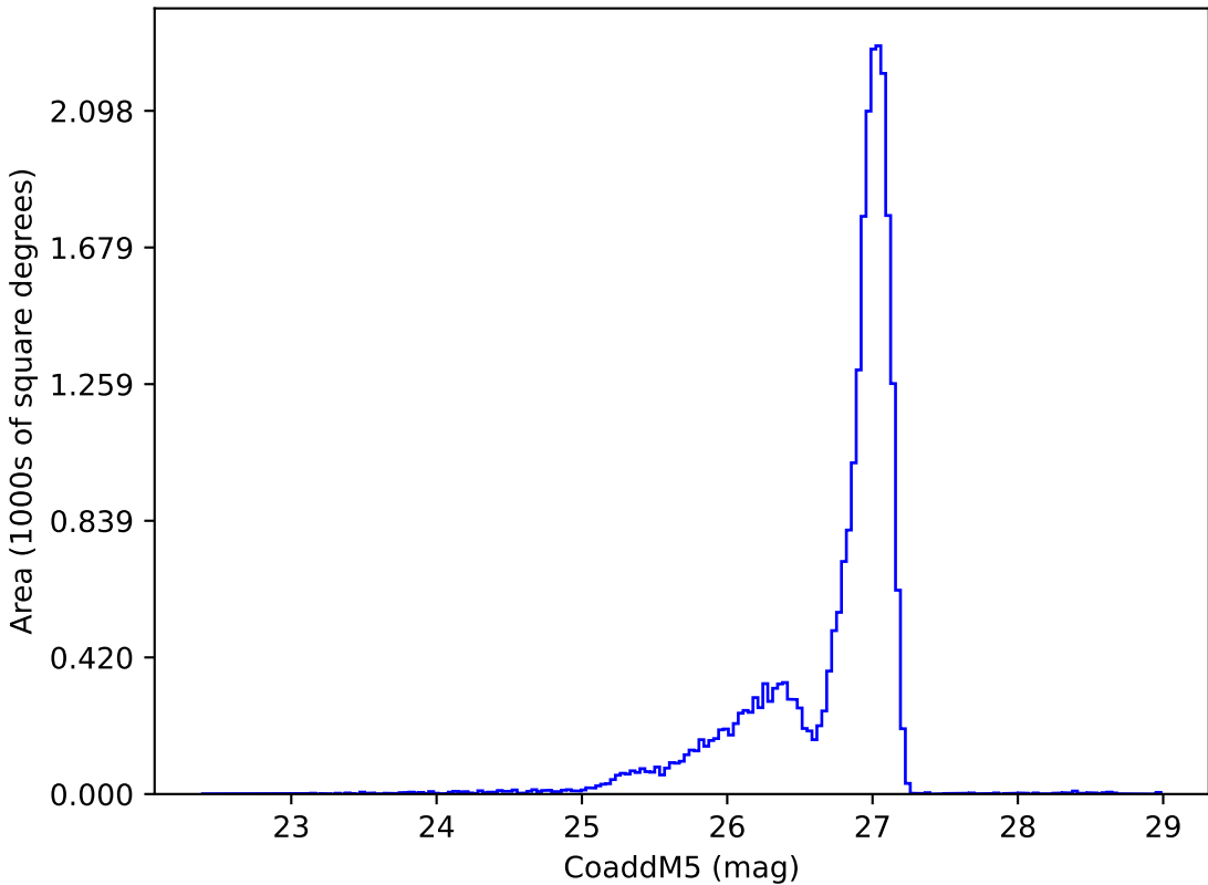
ddf_acor_sf10_lsf15_lsr10_v3.4_10yrs r: CoaddM5
