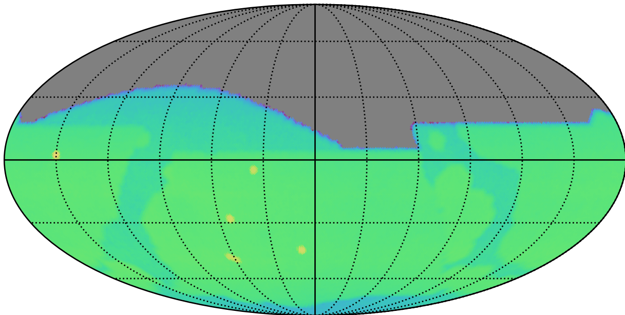
ddf_acor_sf10_lsf15_lsr10_v3.4_10yrs : CoaddM5
