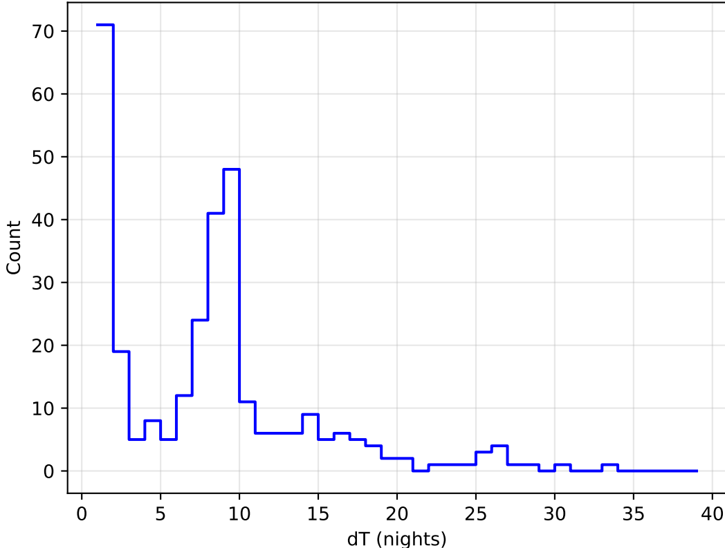
ddf_acor_sf10_lsf15_lsr10_v3.4_10yrs all bands: DD:XMM_LSS Delta Nights Histogram
