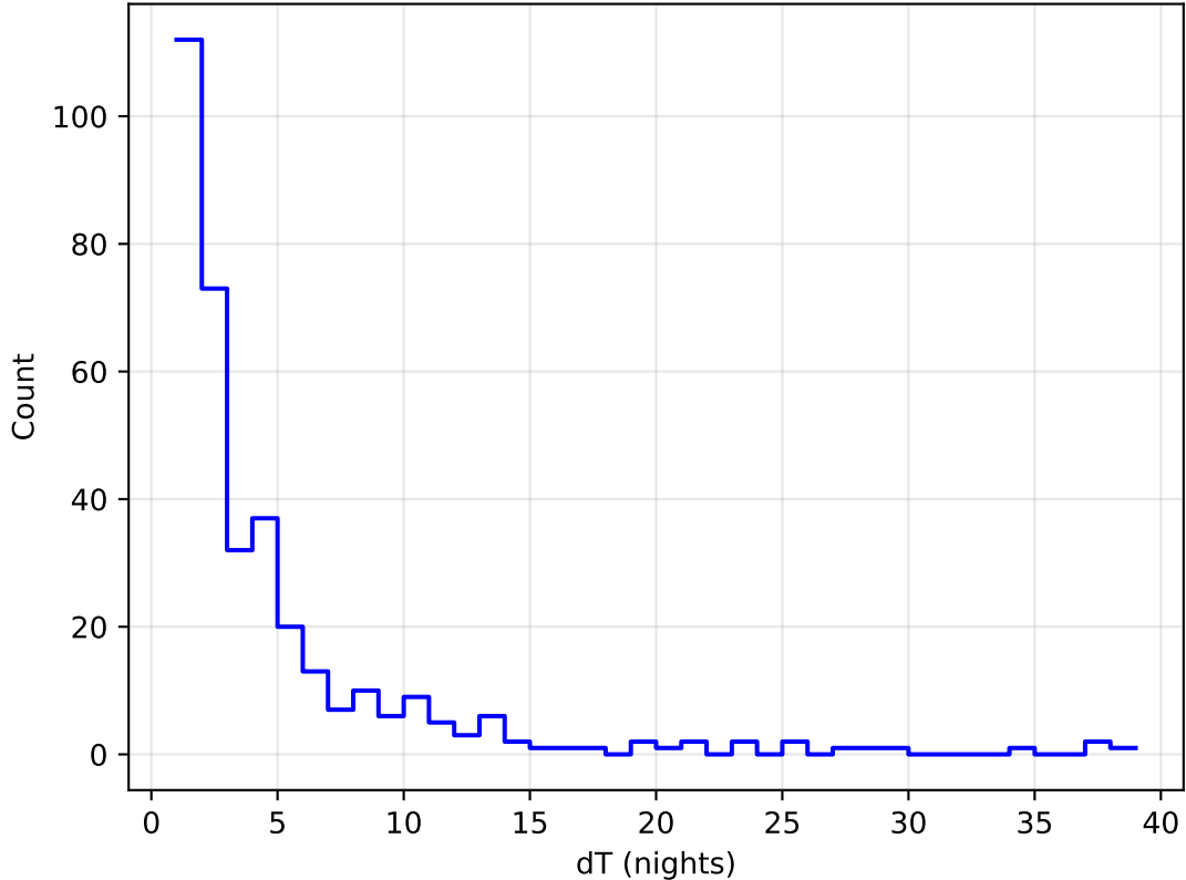
ddf_acor_sf10_lsf15_lsr10_v3.4_10yrs all bands: DD:WFD Delta Nights Histogram
