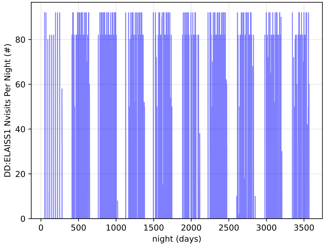
ddf_acor_sf10_lsf15_lsr10_v3.4_10yrs all bands: DD:ELAISS1 Nvisits Per Night
