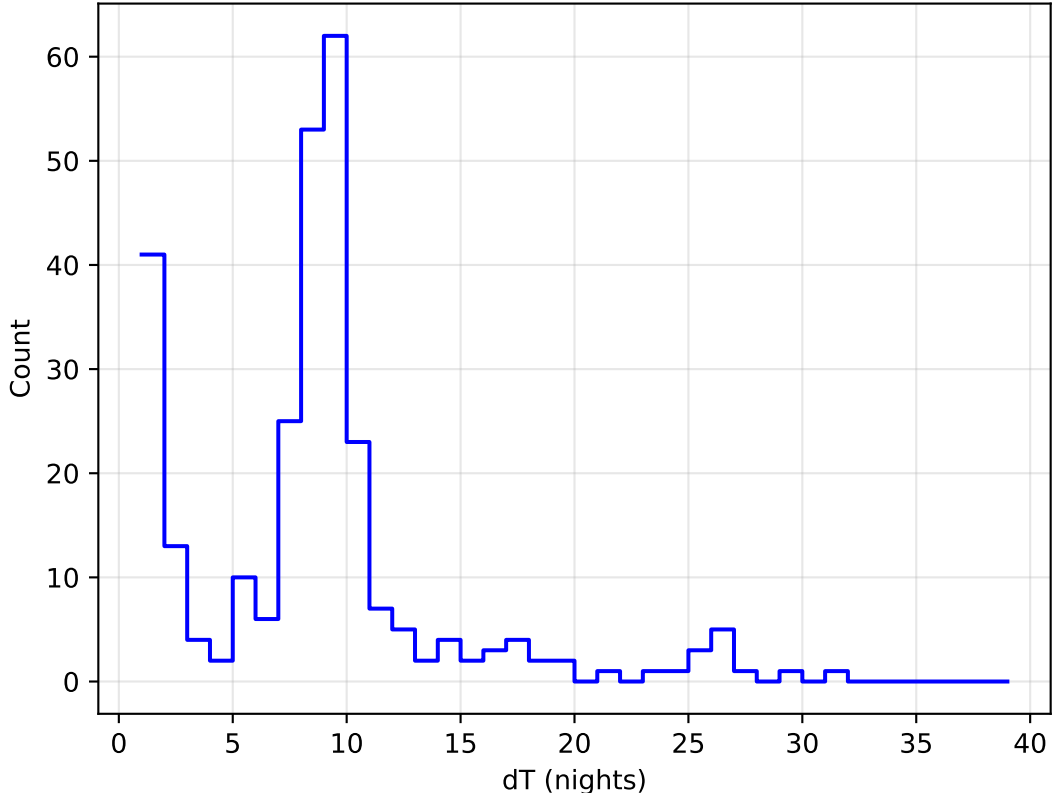
ddf_acor_sf10_lsf15_lsr10_v3.4_10yrs all bands: DD:ELAISS1 Delta Nights Histogram
