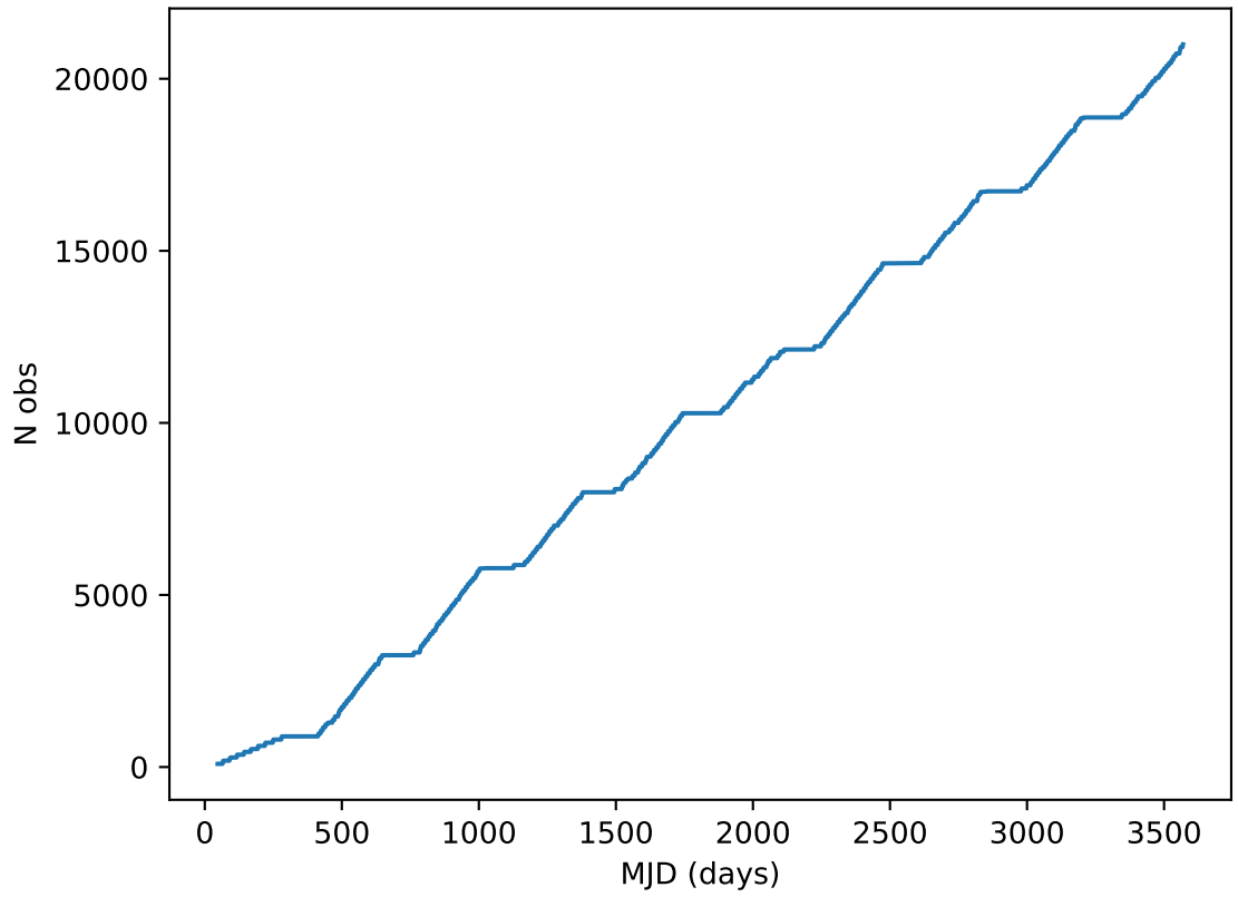
ddf_acor_sf10_ls15_lsr10_v3.4_10yrs all bands: DD:ELAISS1 Cumulative NVisits
