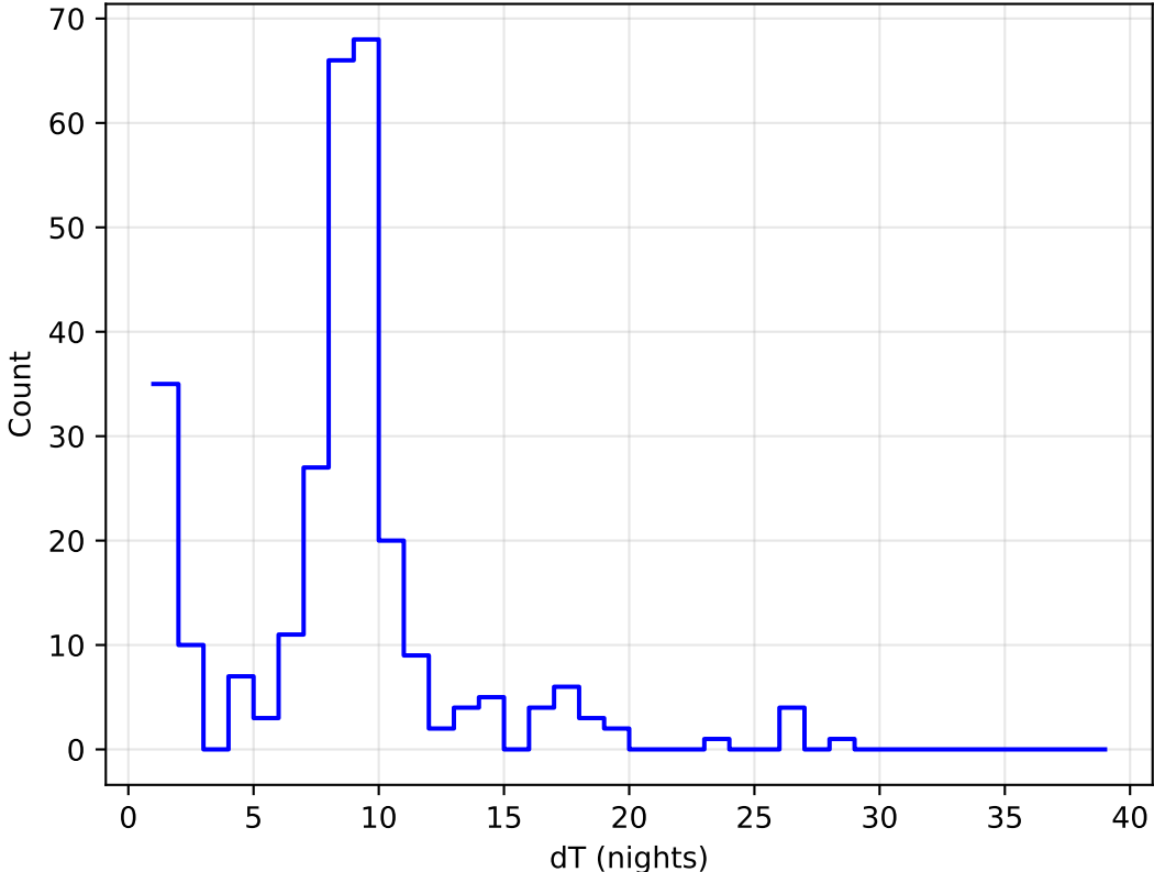
ddf_acor_sf10_lsf15_lsr10_v3.4_10yrs all bands: DD:EDFS Delta Nights Histogram
