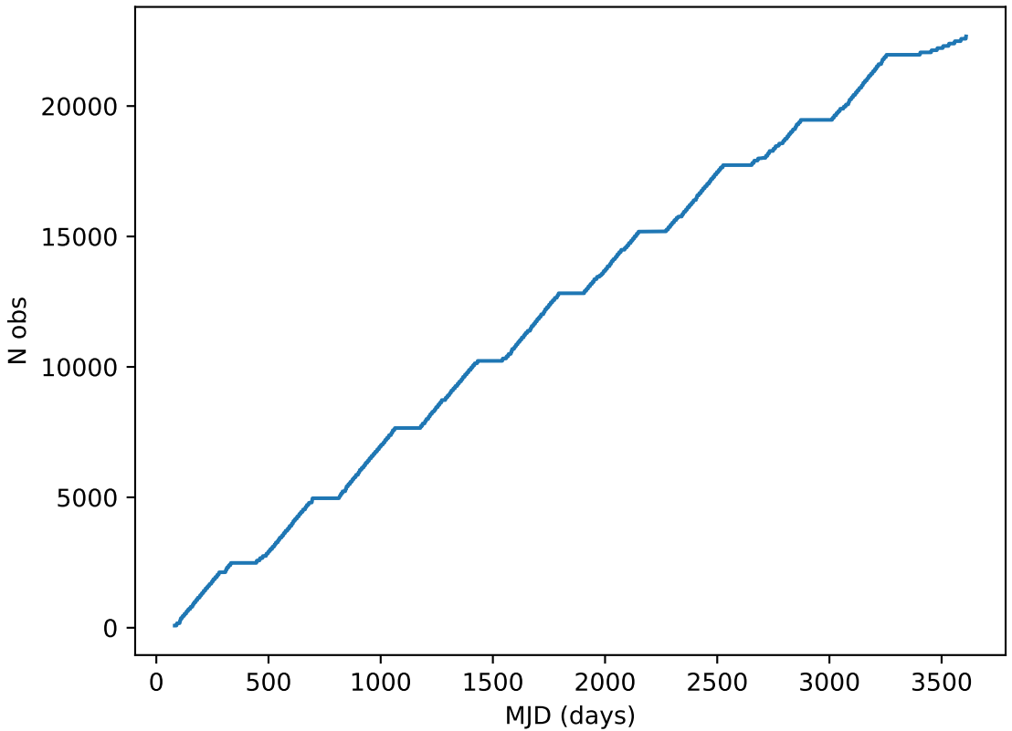
ddf_acor_sf10_lsf15_lsr10_v3.4_10yrs all bands: DD:EDFS Cumulative NVisits
