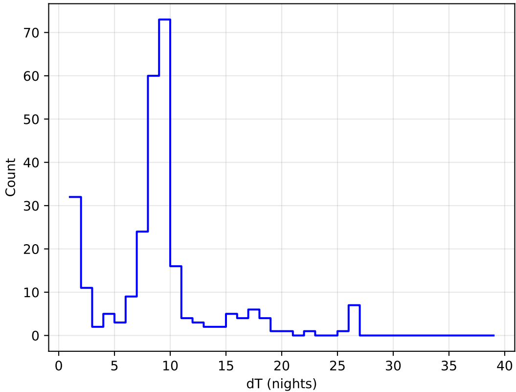
ddf_acor_sf10_lsf15_lsr10_v3.4_10yrs all bands: DD:ECDFS Delta Nights Histogram
