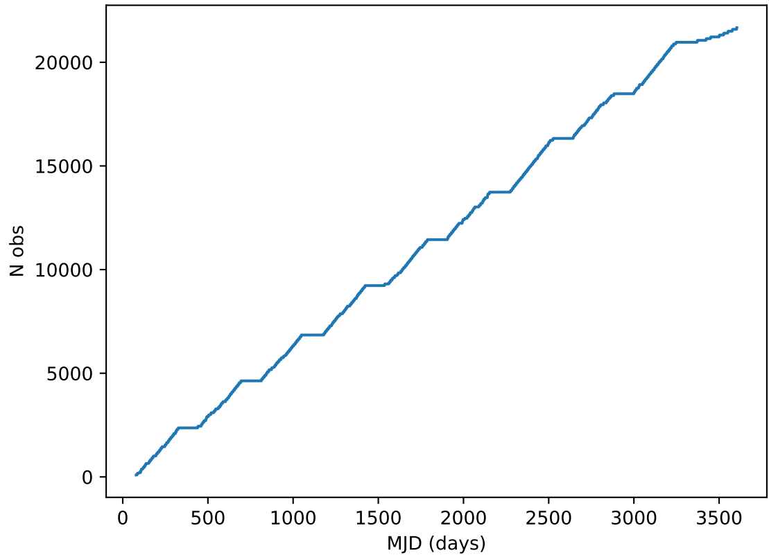
ddf_acor_sf10_lsf15_lsr10_v3.4_10yrs all bands: DD:ECDFS Cumulative NVisits
