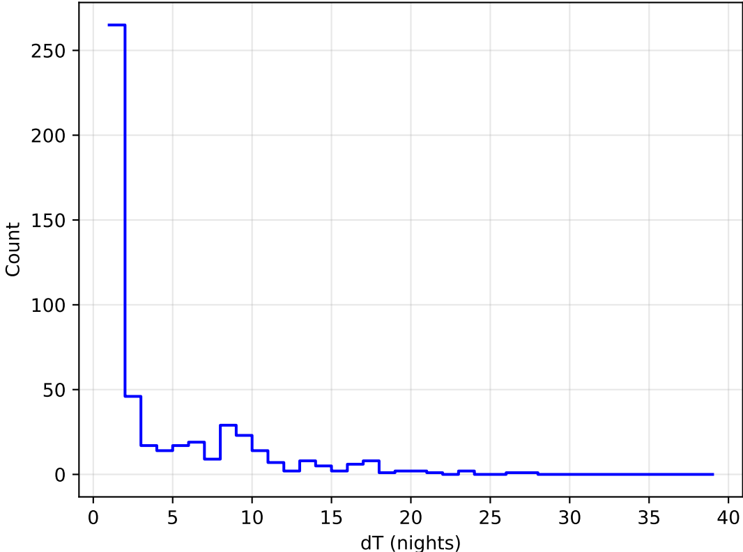
ddf_acor_sf10_Isf15_Isr10_v3.4_10yrs all bands: DD: COSMOS Delta Nights Histogram
