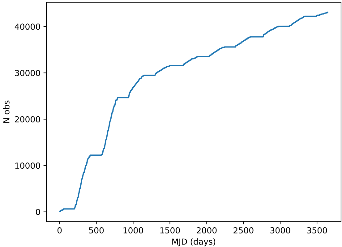
ddf_acor_sf10_lsf15_lsr10_v3.4_10yrs all bands: DD: COSMOS Cumulative NVisits
