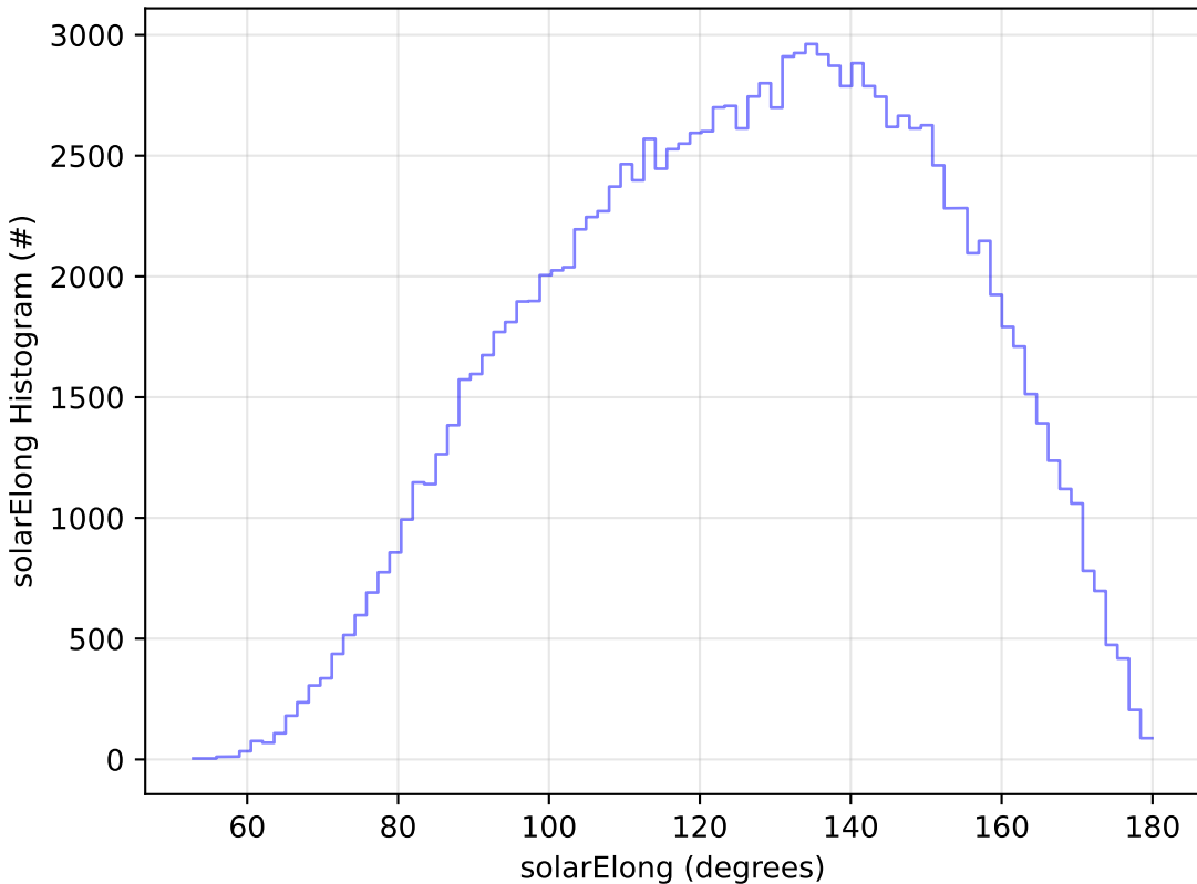
baseline_v3.5_10yrs WFD u band: solarElong Histogram
