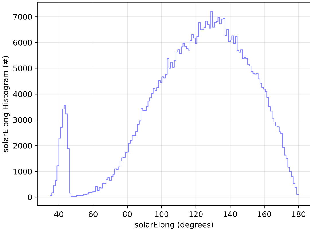
baseline_v3.5_10yrs WFD r band: solarElong Histogram
