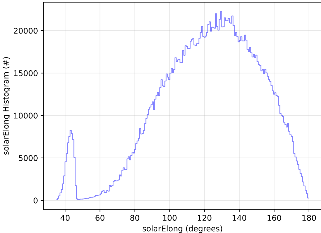
baseline_v3.5_10yrs WFD all bands: solarElong Histogram
